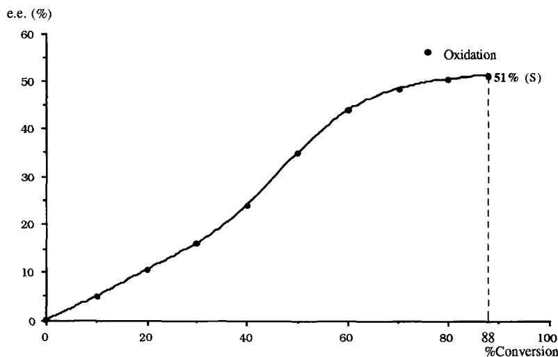
Figure 5 : kinetic resolution
