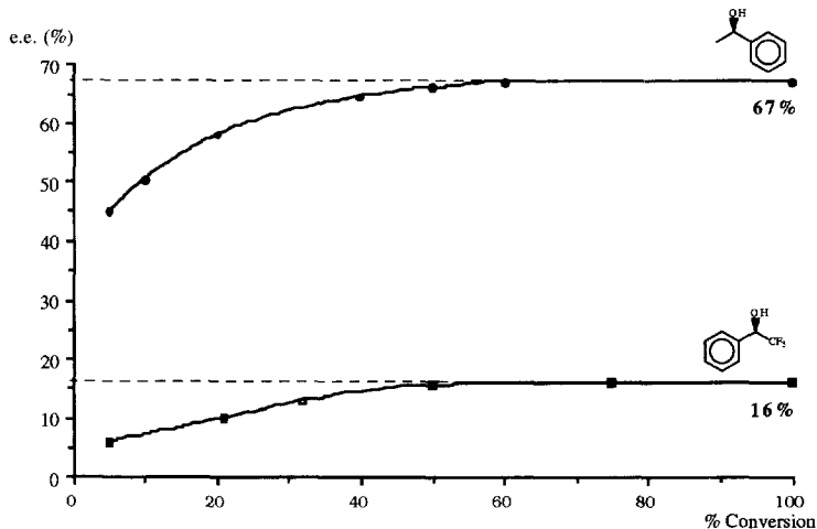
Figure 4 : Evolution of the enantiomeric excesses with the conversion.
