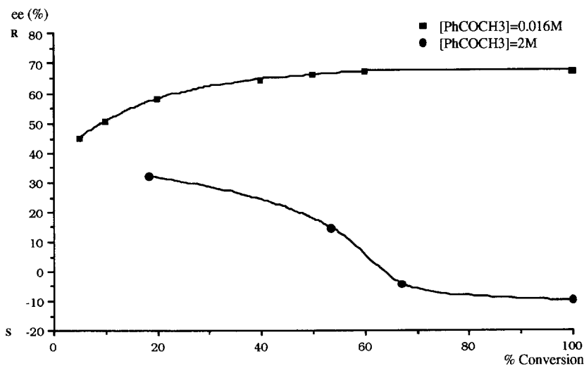
Figure 9 : Reduction of the acetophenone : influence of the substrate concentration on the e.e.. Conditions : [Rh]/[S] = 5%; T = 25°C; 1b /[Rh] = 2; [KOH]/[Rh] = 6.
