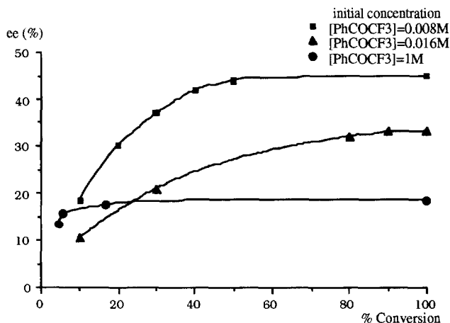
Figure 8 : reduction of the \alpha,\alpha,\alpha -trifluoroacetophenone : influence of the substrate concentration on the e.e..
